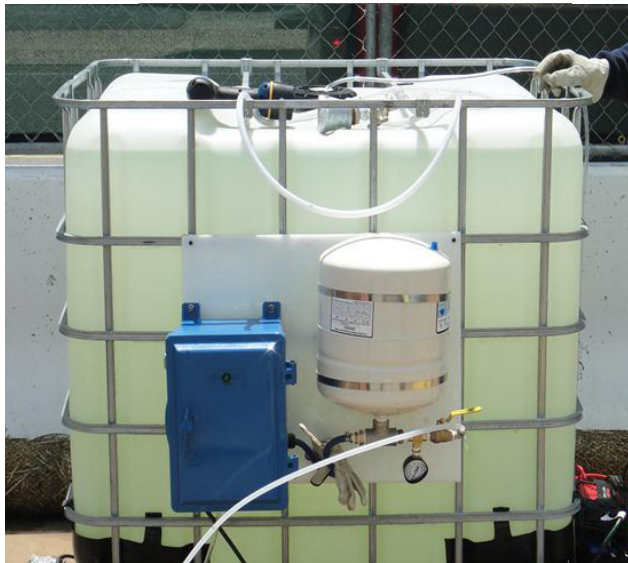
1,000 Liter ESP Solution Tote Bin
