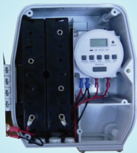
Squirt DC's battery pack and timer nest inside splash resistant cabinet
